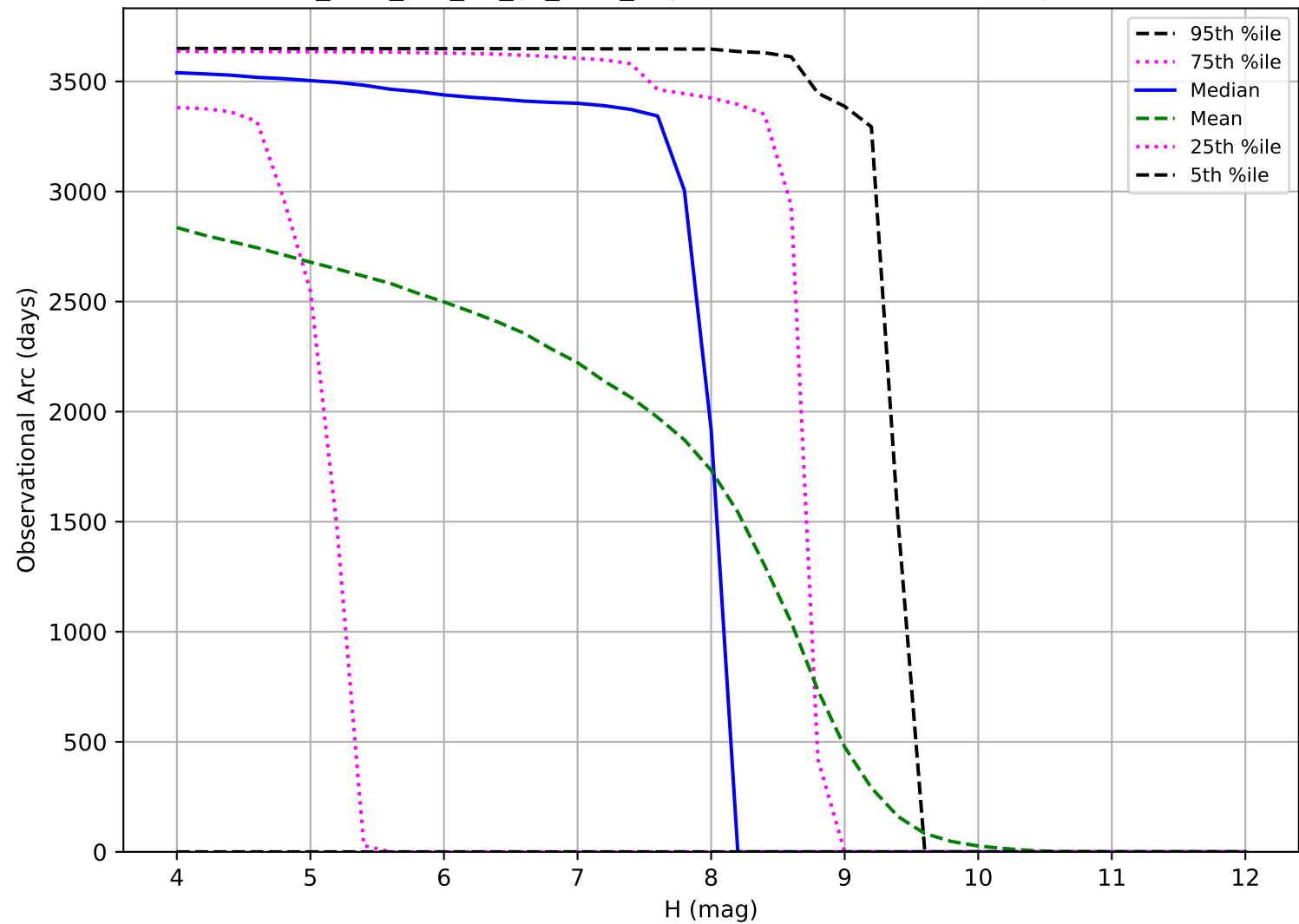
too_elab_r64_d3_gz_v3.4_10yrs: Observational Arc Length TNO
