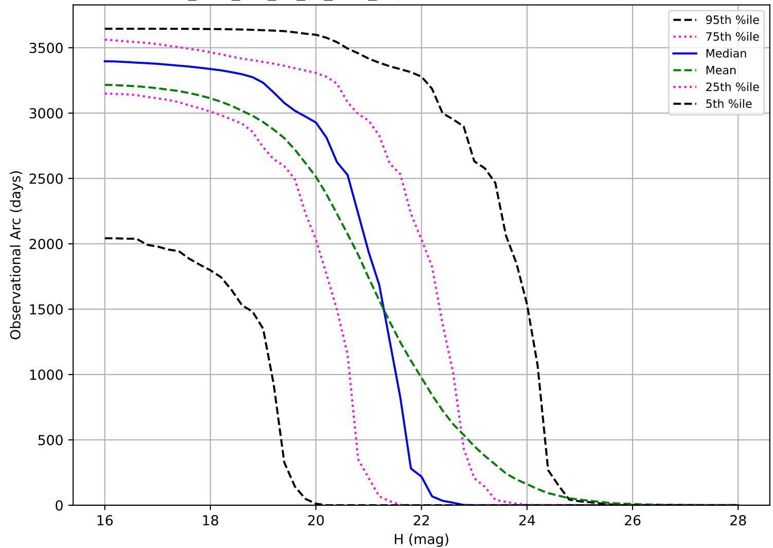
too_elab_r64_d3_gz_v3.4_10yrs: Observational Arc Length PHA
