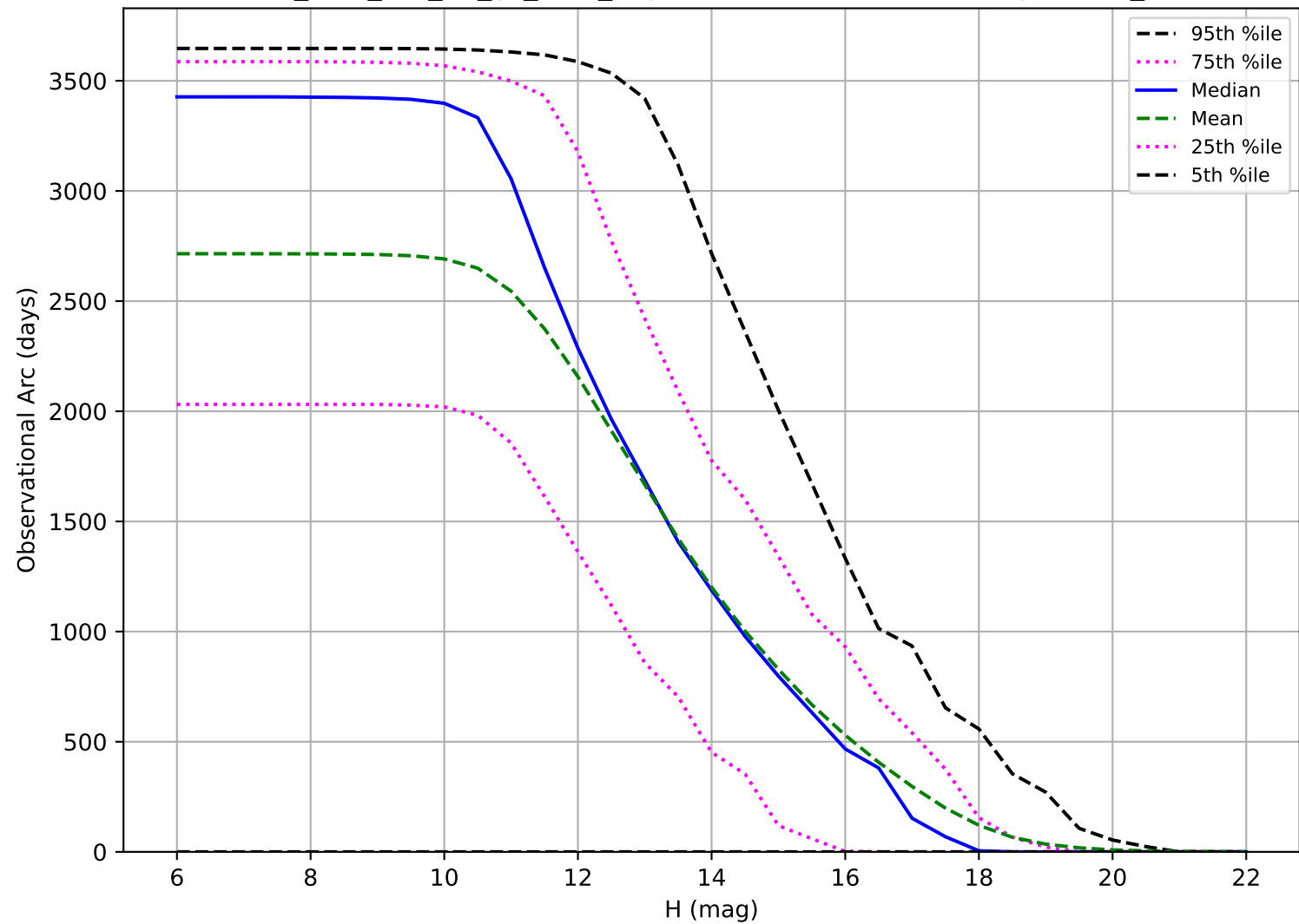
too_elab_r64_d3_gz_v3.4_10yrs: Observational Arc Length OCC_r5
