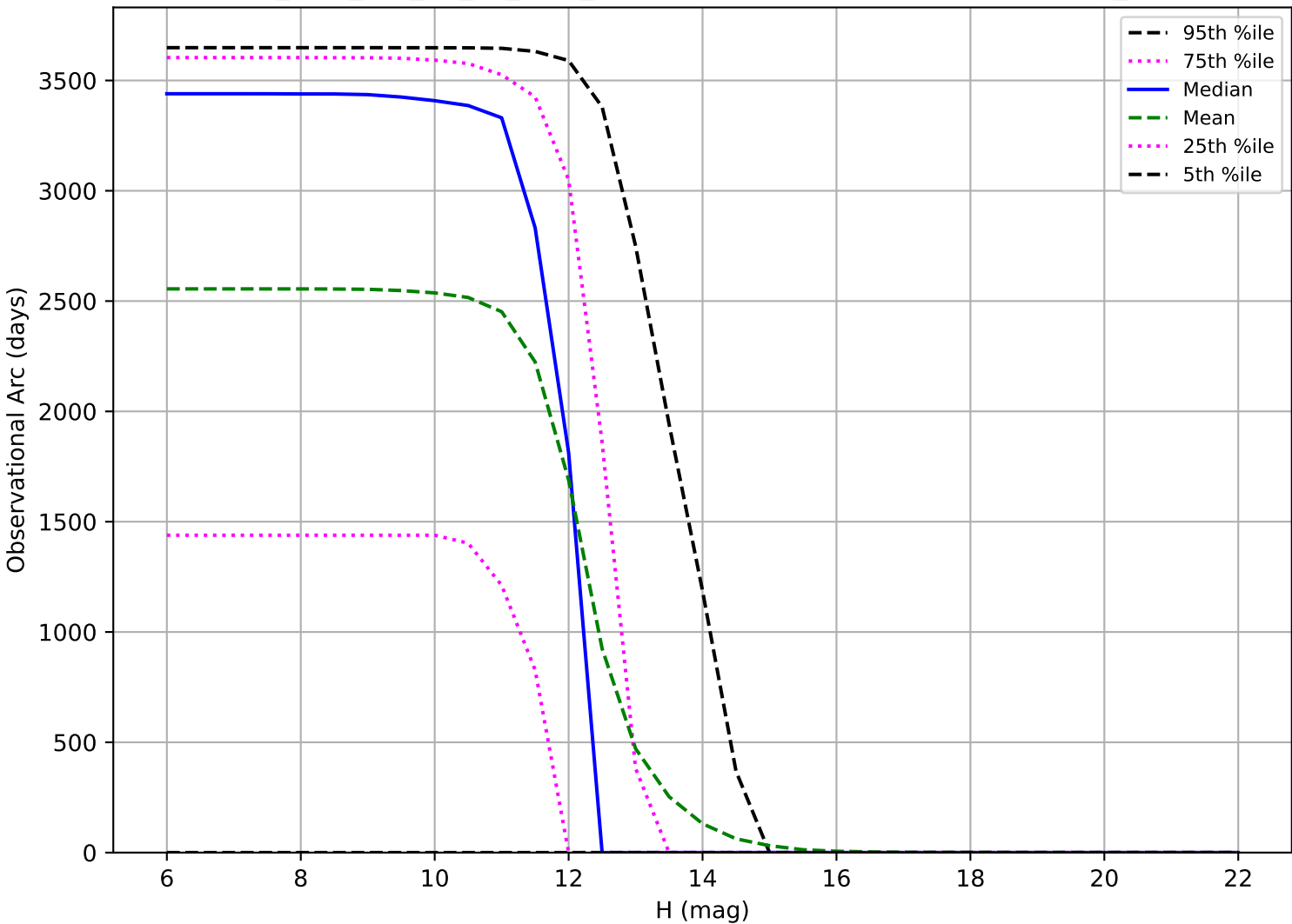
too_elab_r64_d3_gz_v3.4_10yrs: Observational Arc Length OCC_r20
