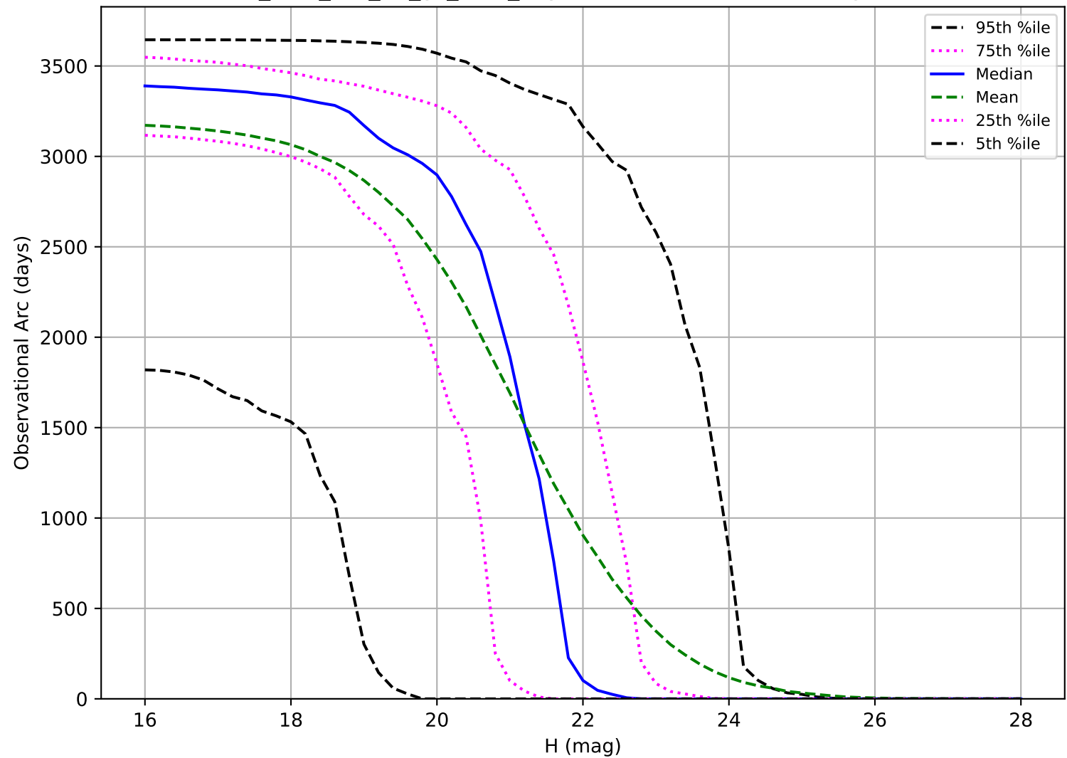
too_elab_r64_d3_gz_v3.4_10yrs: Observational Arc Length NEO
