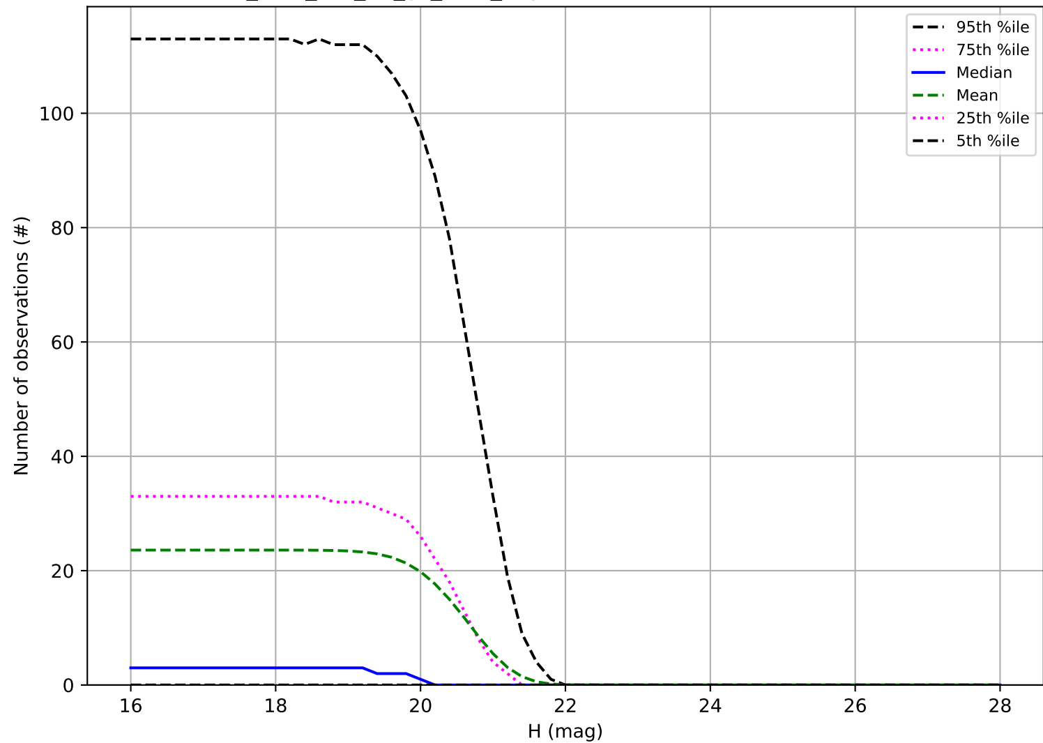
too_elab_r64_d3_gz_v3.4_10yrs: Number of observations Vatira
