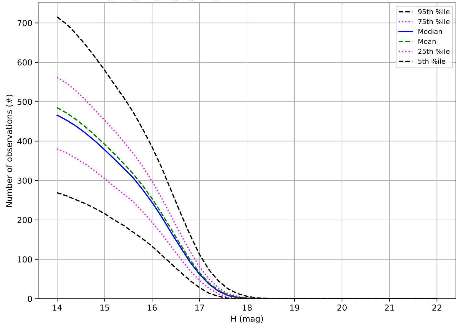
too_elab_r64_d3_gz_v3.4_10yrs: Number of observations Trojan
