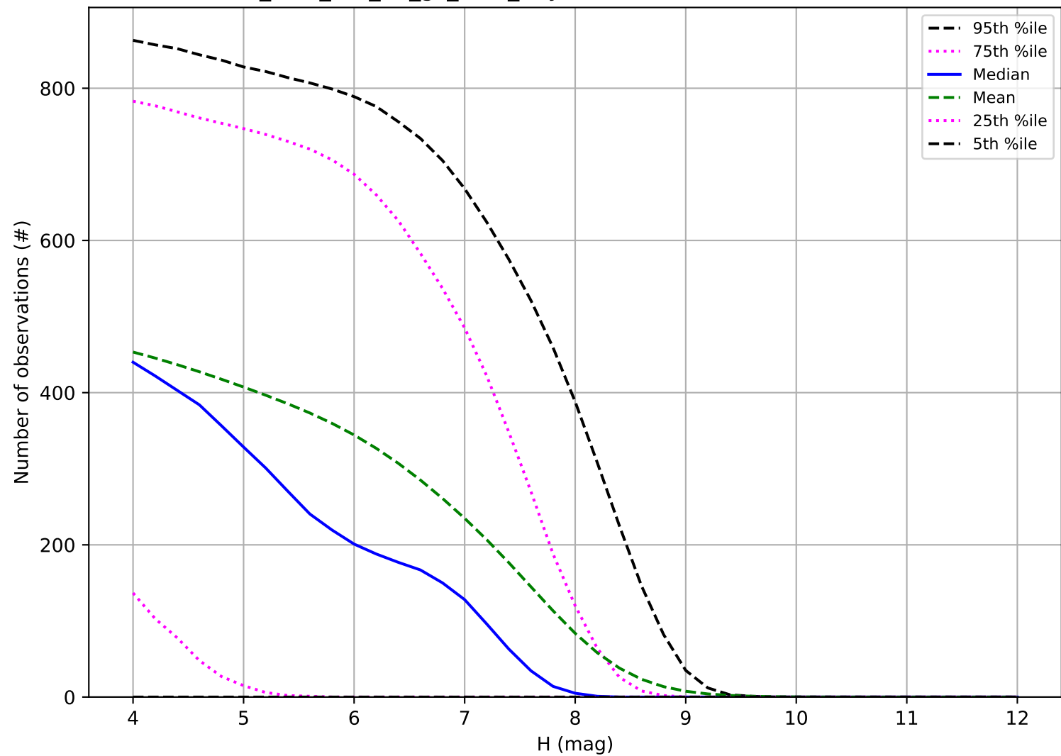
too_elab_r64_d3_gz_v3.4_10yrs: Number of observations TNO
