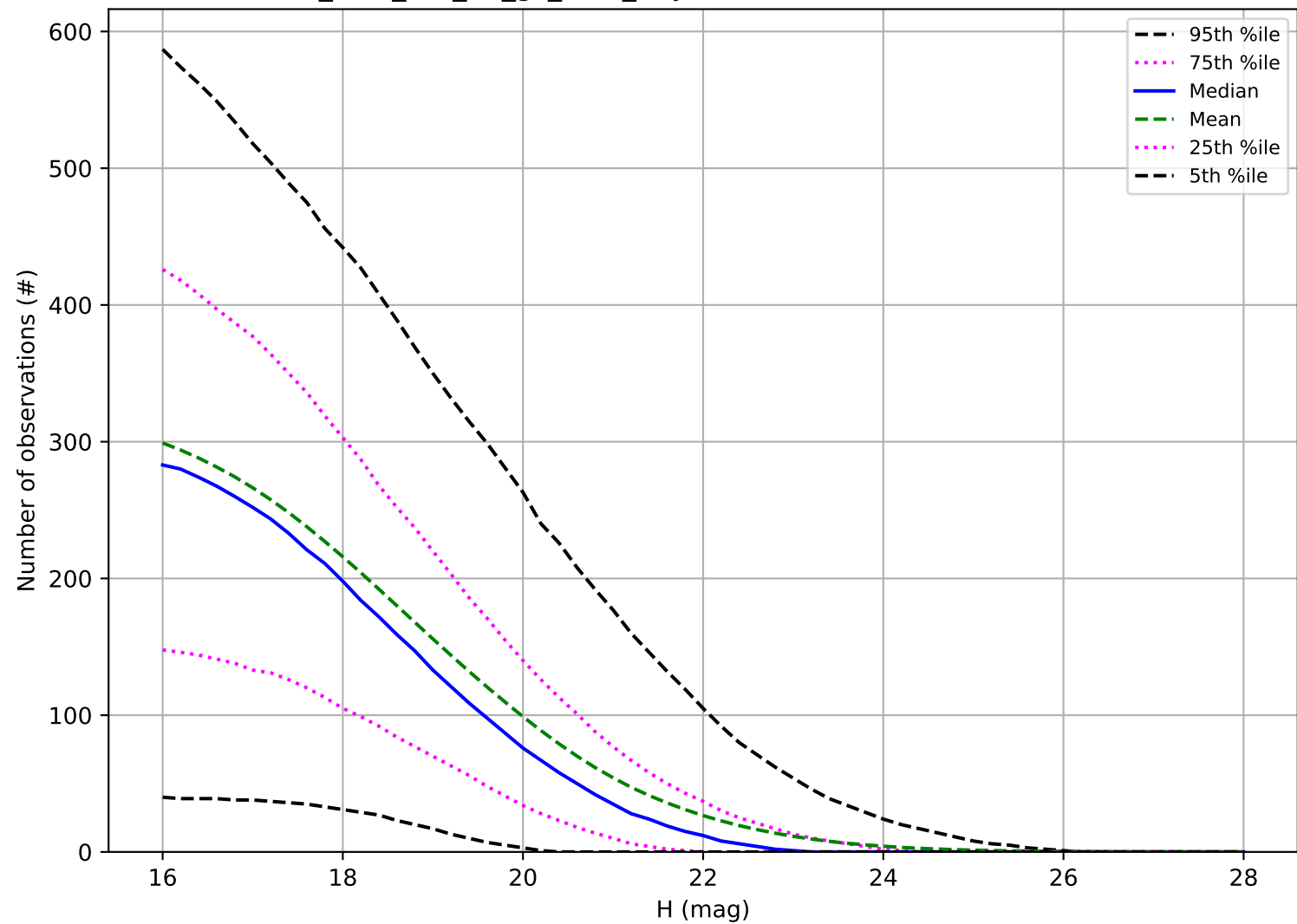
too_elab_r64_d3_gz_v3.4_10yrs: Number of observations PHA
