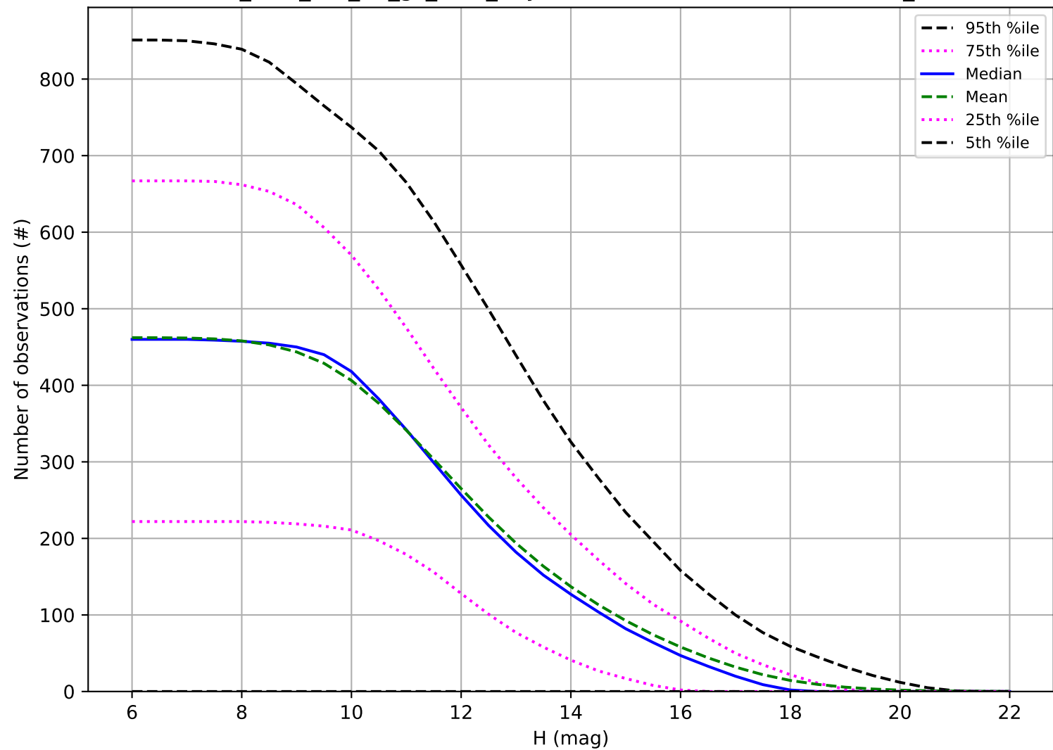
too_elab_r64_d3_gz_v3.4_10yrs: Number of observations OCC_r5
