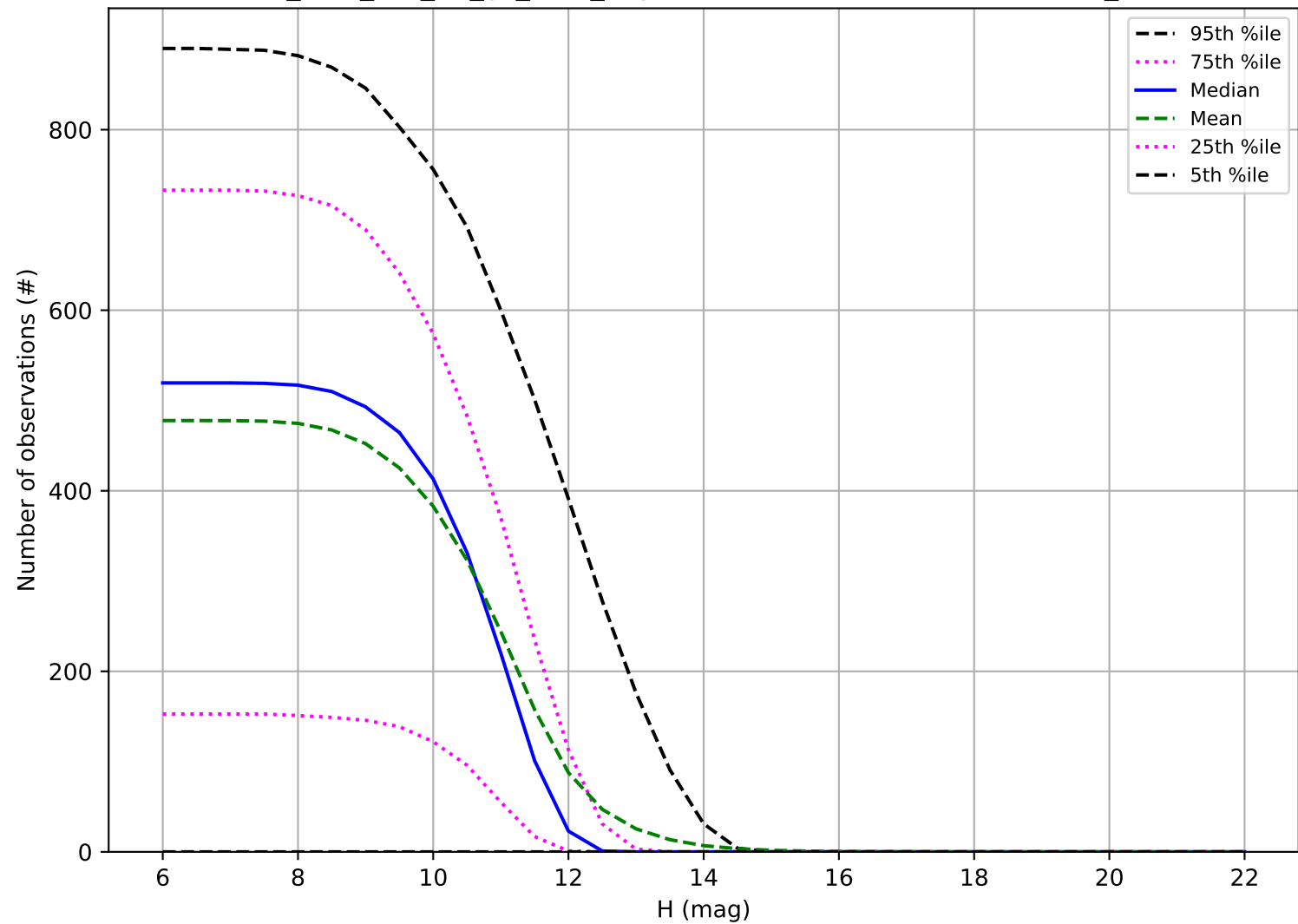
too_elab_r64_d3_gz_v3.4_10yrs: Number of observations OCC_r20
