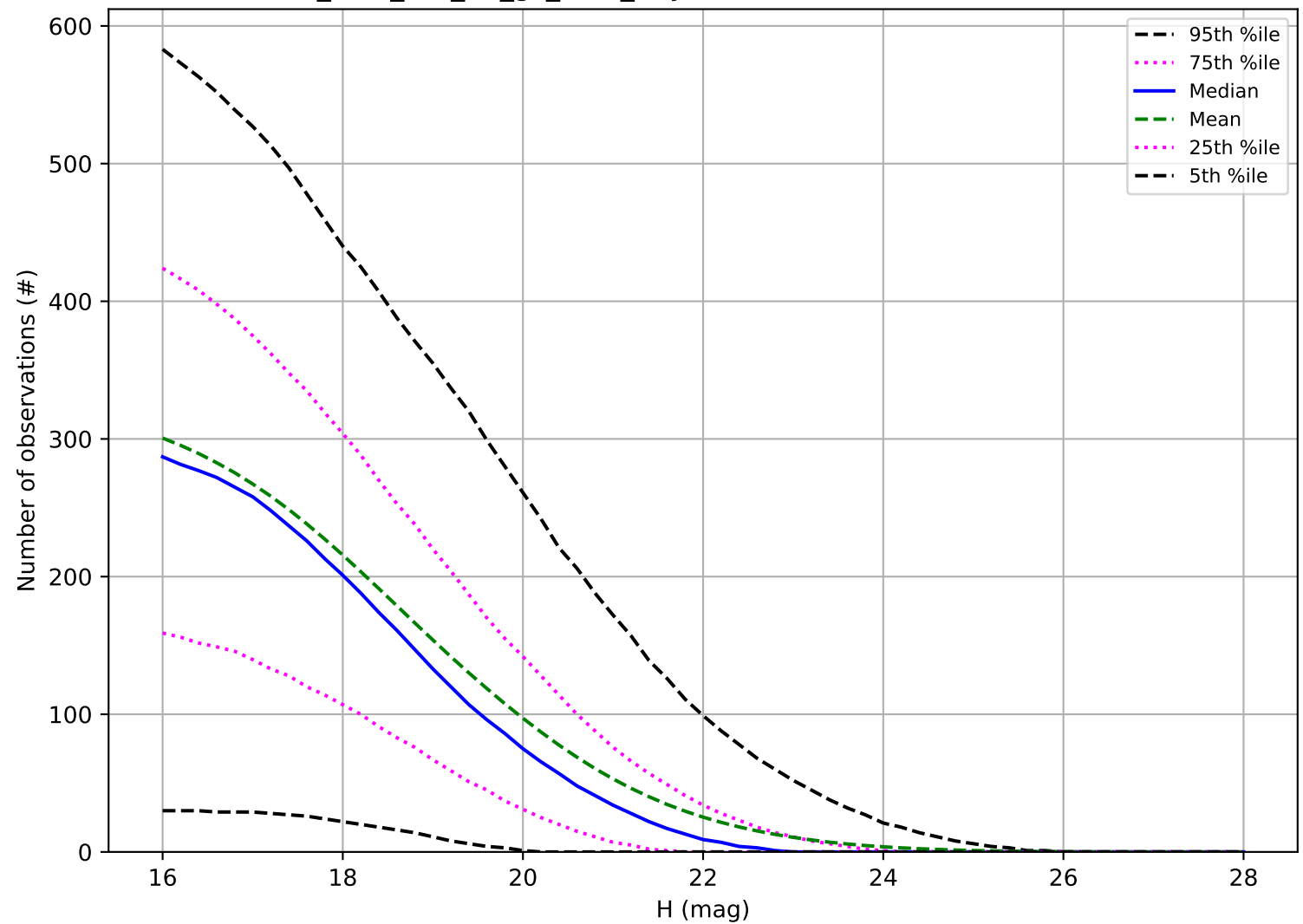
too_elab_r64_d3_gz_v3.4_10yrs: Number of observations NEO
