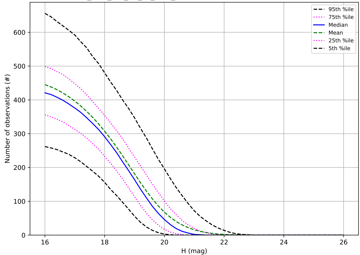
too_elab_r64_d3_gz_v3.4_10yrs: Number of observations MBA
