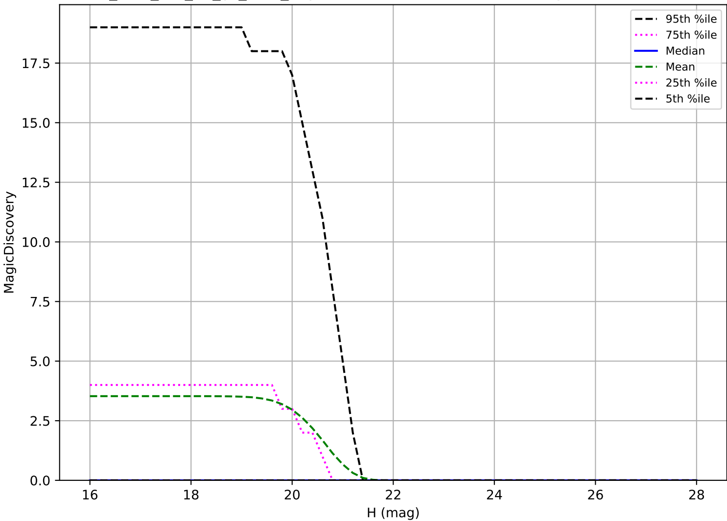
too_elab_r64_d3_gz_v3.4_10yrs: Vatira 6 detections in 60 nights detection loss
