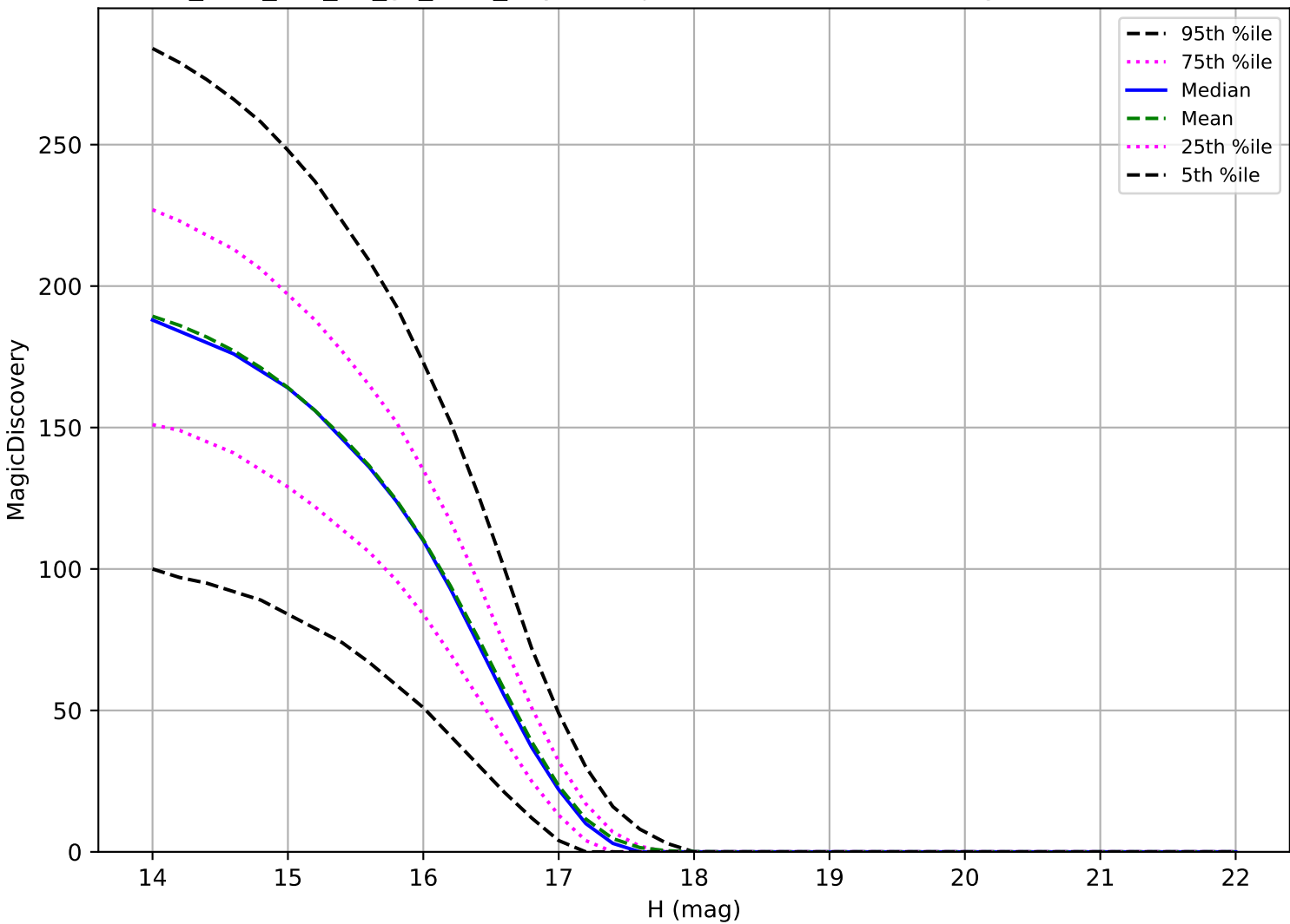
too_elab_r64_d3_gz_v3.4_10yrs: Trojan 6 detections in 60 nights detection loss
