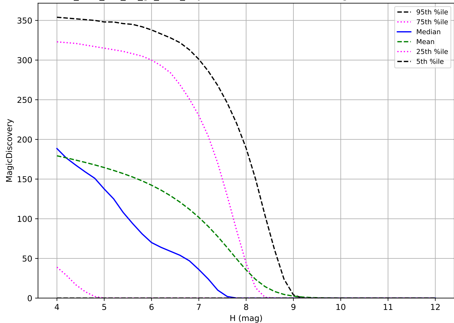
too_elab_r64_d3_gz_v3.4_10yrs: TNO 6 detections in 60 nights detection loss
