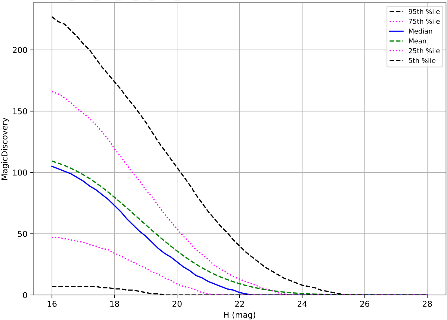
too_elab_r64_d3_gz_v3.4_10yrs: PHA 6 detections in 60 nights detection loss
