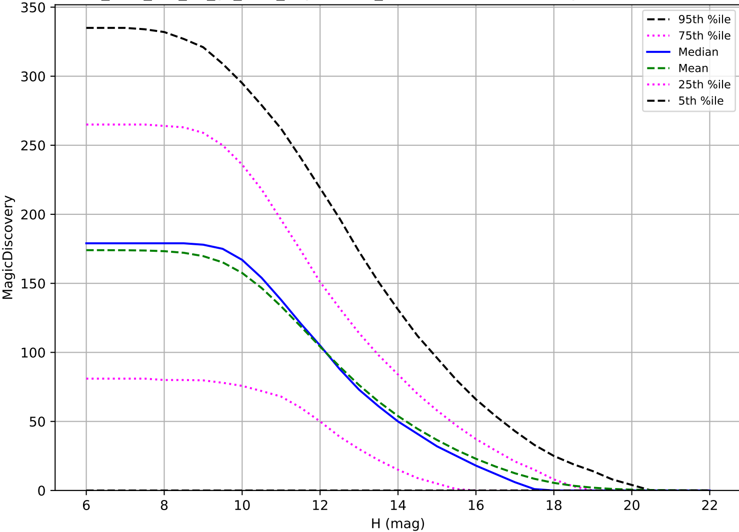
too_elab_r64_d3_gz_v3.4_10yrs: OCC_r5 6 detections in 60 nights detection loss
