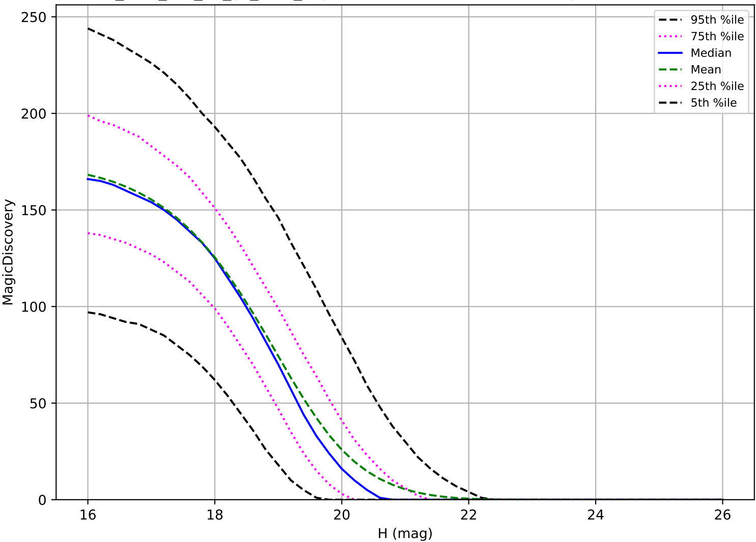
too_elab_r64_d3_gz_v3.4_10yrs: MBA 6 detections in 60 nights detection loss
