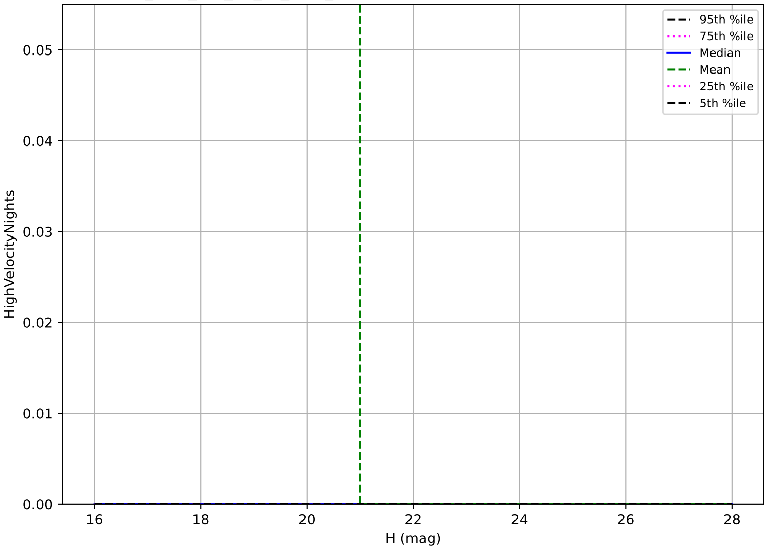
too_elab_r64_d3_gz_v3.4_10yrs: Vatira High velocity pair detection loss
