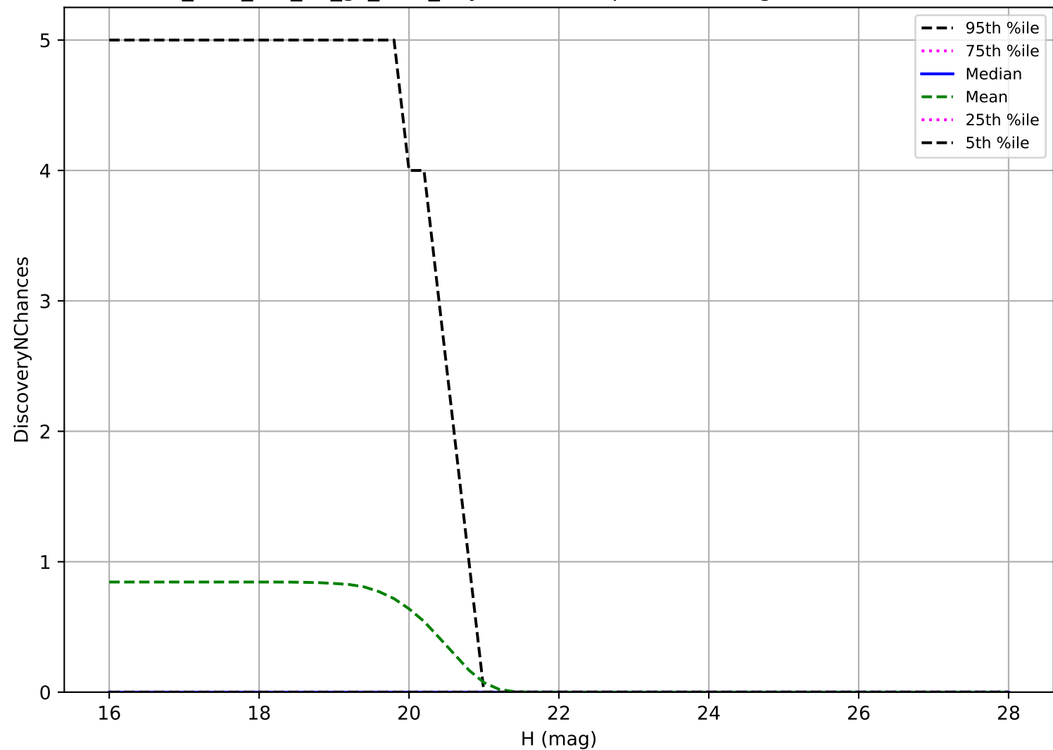
too_elab_r64_d3_gz_v3.4_10yrs: Vatira 3 pairs in 15 nights detection loss
