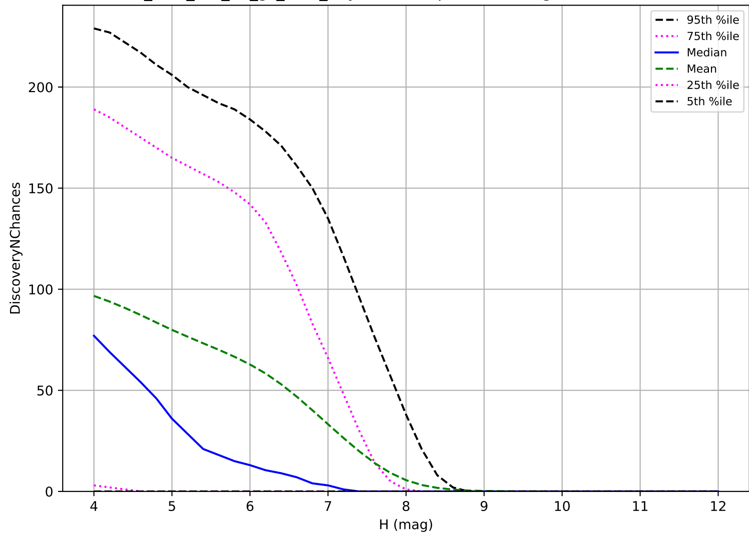
too_elab_r64_d3_gz_v3.4_10yrs: TNO 3 pairs in 15 nights detection loss
