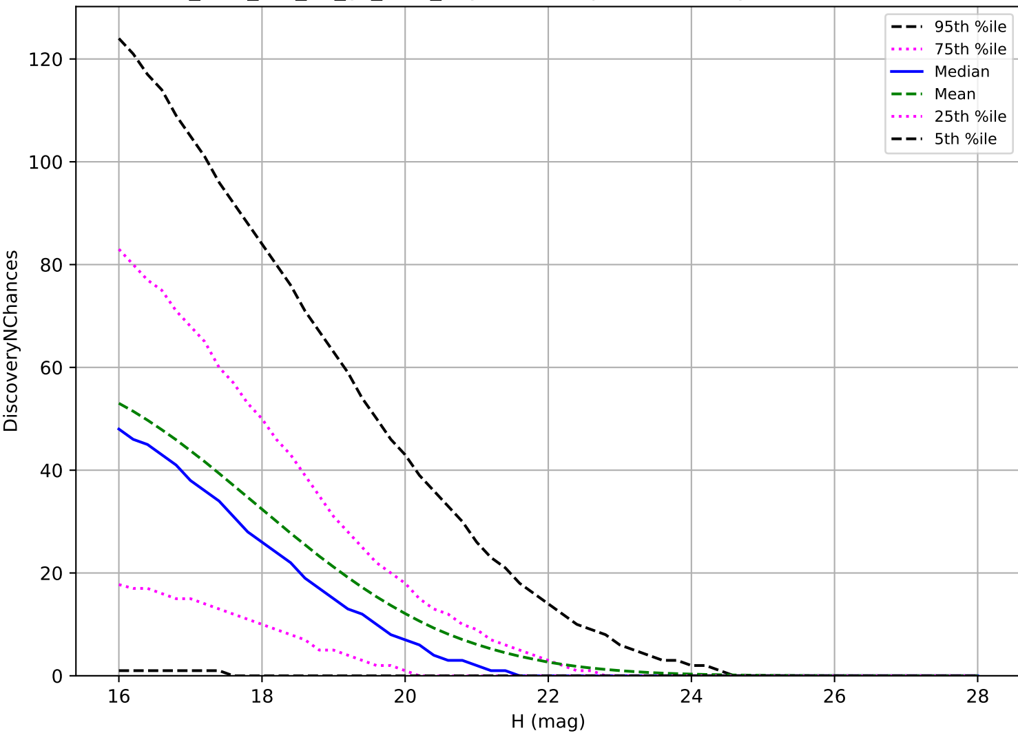
too_elab_r64_d3_gz_v3.4_10yrs: PHA 3 pairs in 15 nights detection loss
