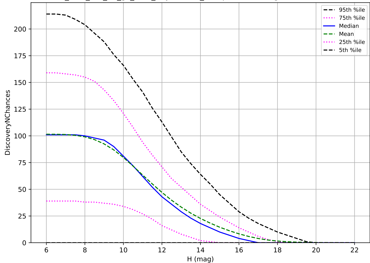
too_elab_r64_d3_gz_v3.4_10yrs: OCC_r5 3 pairs in 15 nights detection loss
