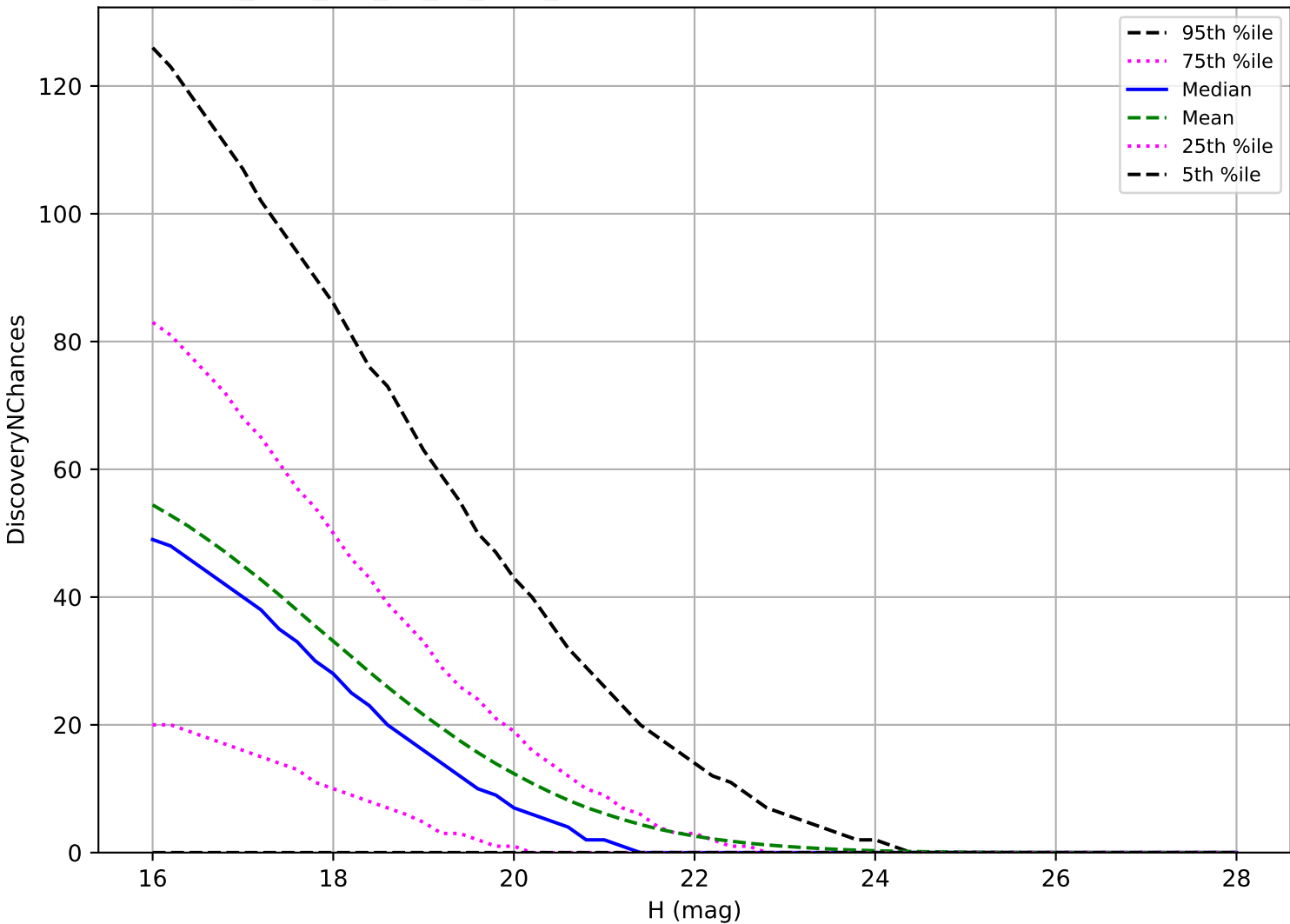
too_elab_r64_d3_gz_v3.4_10yrs: NEO 3 pairs in 15 nights detection loss
