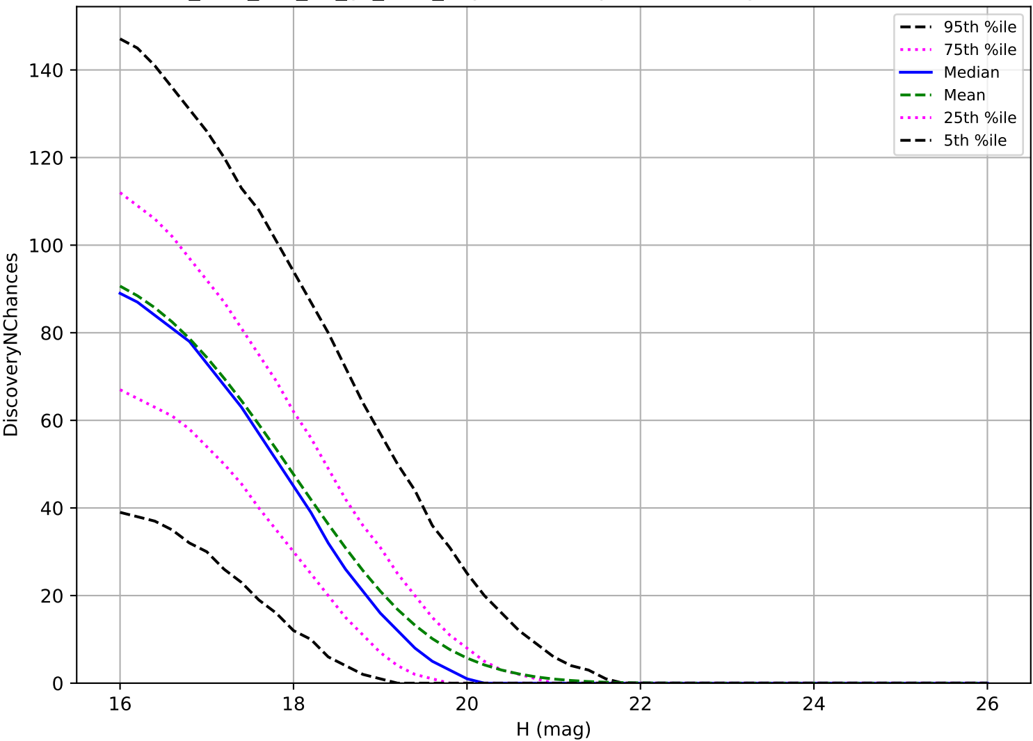
too_elab_r64_d3_gz_v3.4_10yrs: MBA 3 pairs in 15 nights detection loss
