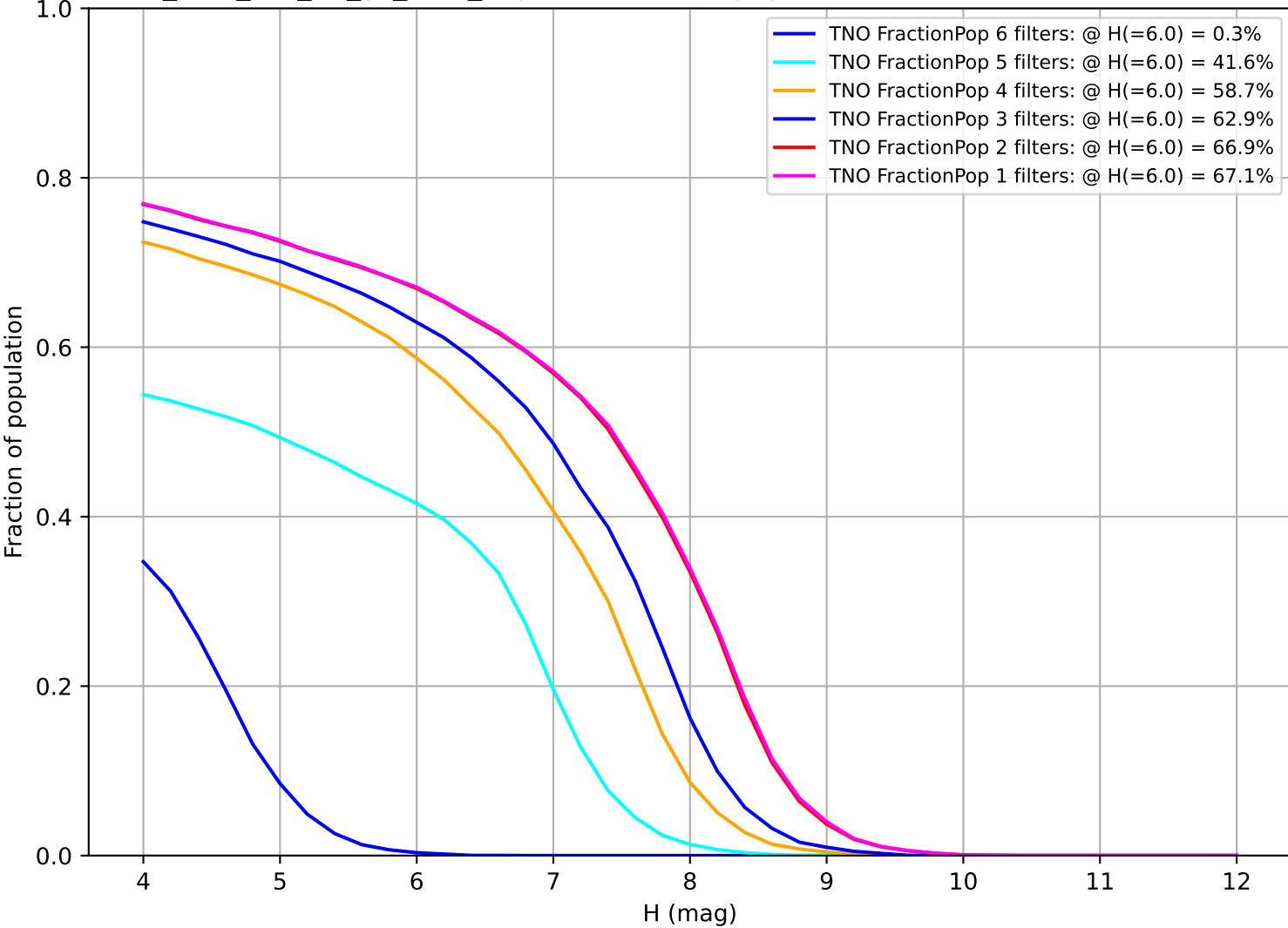
too_elab_r64_d3_gz_v3.4_10yrs: Fraction of population with colors in X filters TNO
