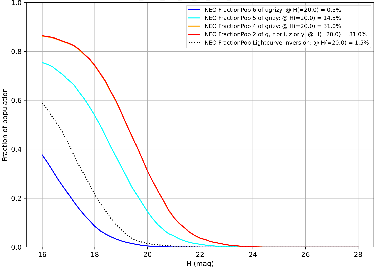
too_elab_r64_d3_gz_v3.4_10yrs NEO
