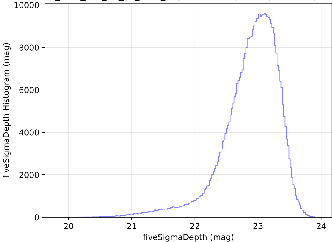
too_elab_r64_d3_gz_v3.4_10yrs z: fiveSigmaDepth Histogram
