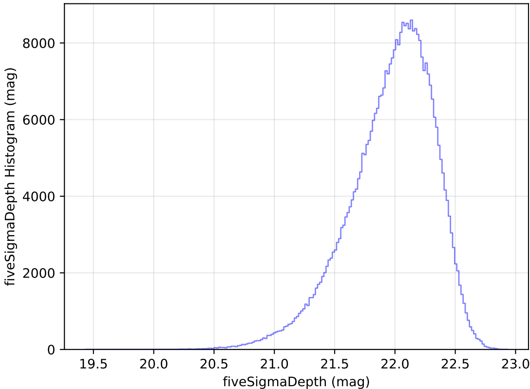
too_elab_r64_d3_gz_v3.4_10yrs y: fiveSigmaDepth Histogram
