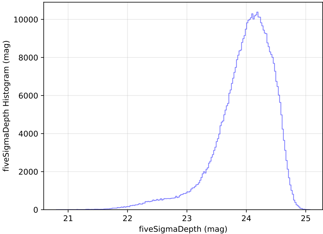
too_elab_r64_d3_gz_v3.4_10yrs r: fiveSigmaDepth Histogram
