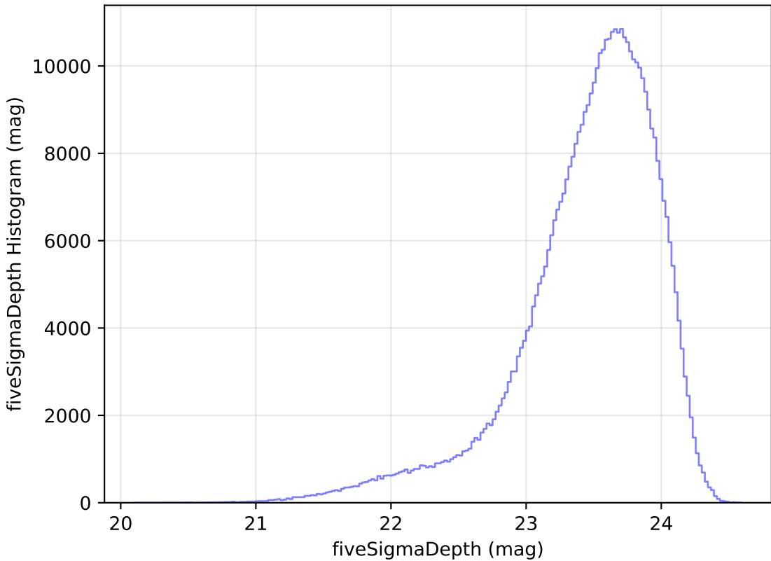
too_elab_r64_d3_gz_v3.4_10yrs i: fiveSigmaDepth Histogram
