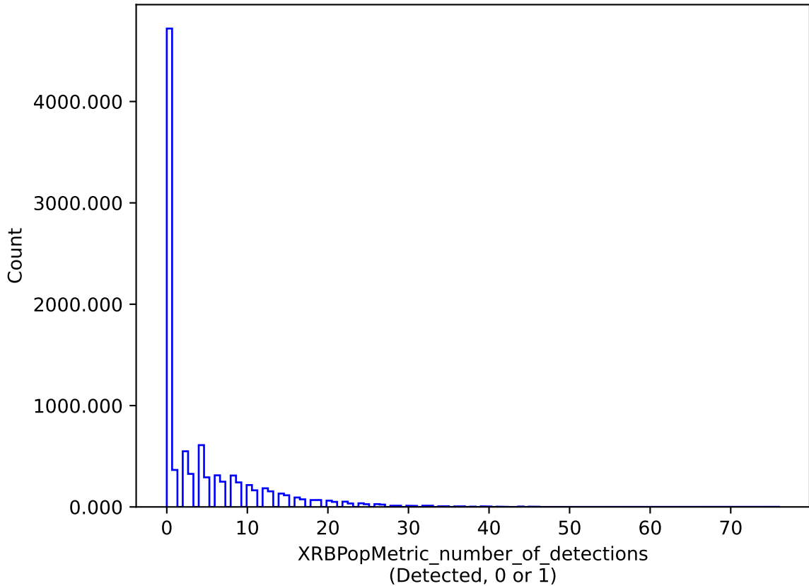
too_elab_r64_d3_gz_v3.4_10yrs : XRBPoMetric_number_of_detections
