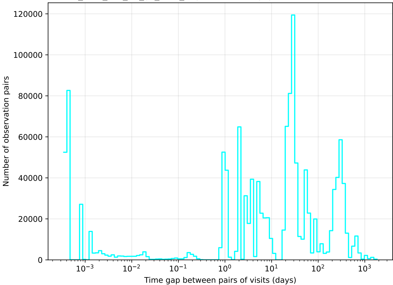
too_elab_r64_d3_gz_v3.4_10yrs u band: Tgaps observationStartMJD
