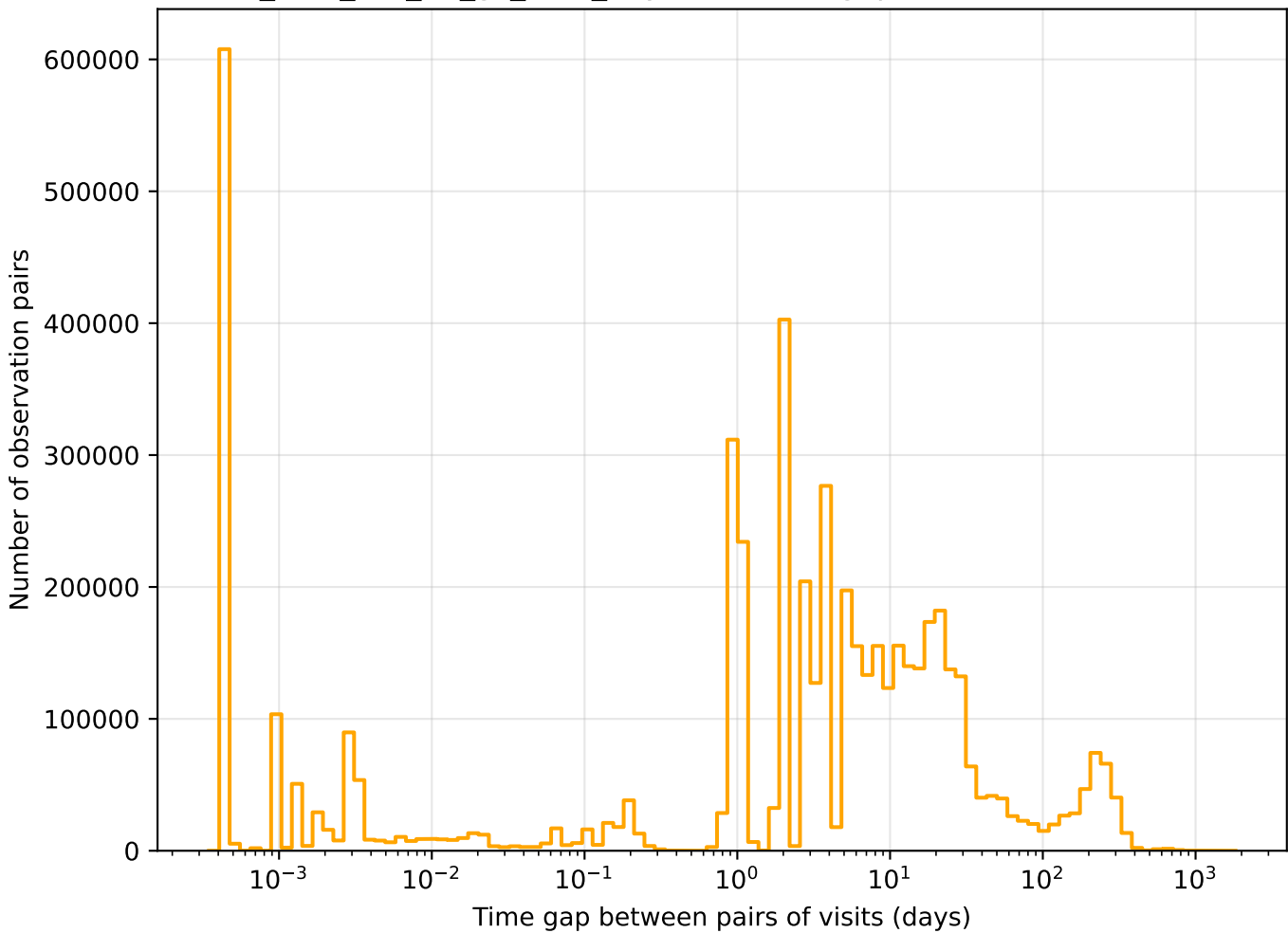
too_elab_r64_d3_gz_v3.4_10yrs r band: Tgaps observationStartMJD
