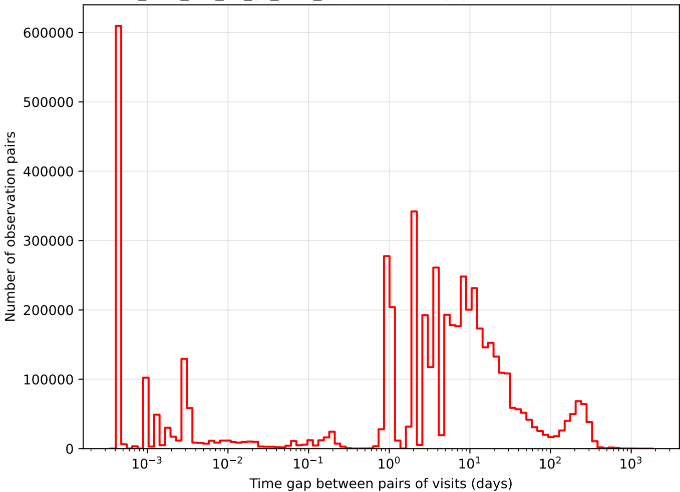
too_elab_r64_d3_gz_v3.4_10yrs i band: Tgaps observationStartMJD
