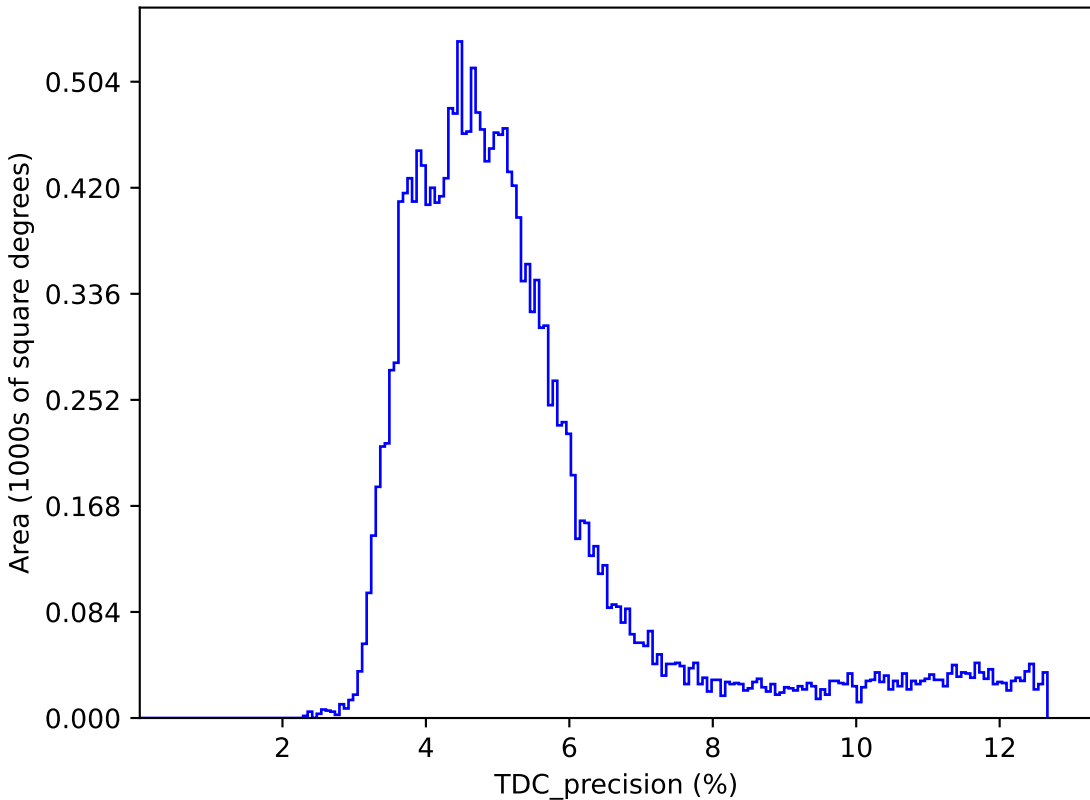
too_elab_r64_d3_gz_v3.4_10yrs : TDC_precision
