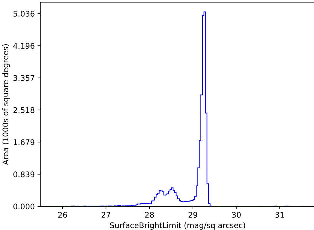
too_elab_r64_d3_gz_v3.4_10yrs z: SurfaceBrightLimit
