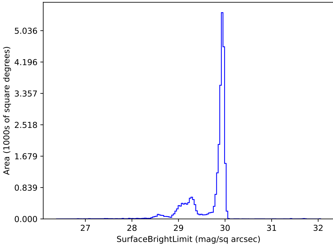
too_elab_r64_d3_gz_v3.4_10yrs i: SurfaceBrightLimit
