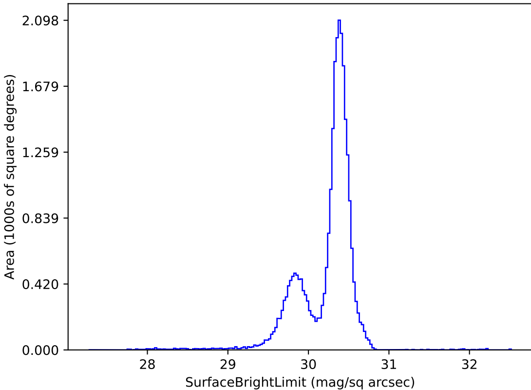
too_elab_r64_d3_gz_v3.4_10yrs g: SurfaceBrightLimit
