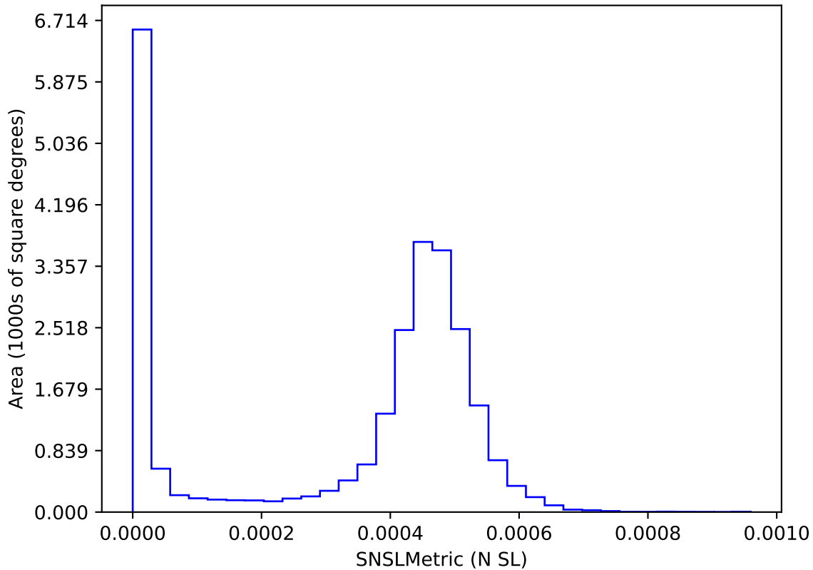
too_elab_r64_d3_gz_v3.4_10yrs : SNSLMetric
