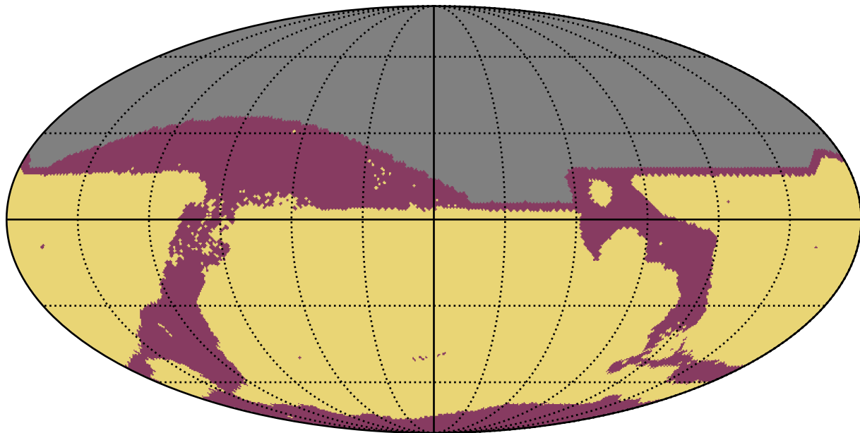
too_elab_r64_d3_gz_v3.4_10yrs : RapidRevisits
