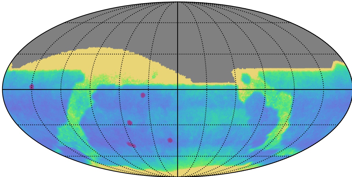
too_elab_r64_d3_gz_v3.4_10yrs : Proper Motion Uncert @ 24.0
