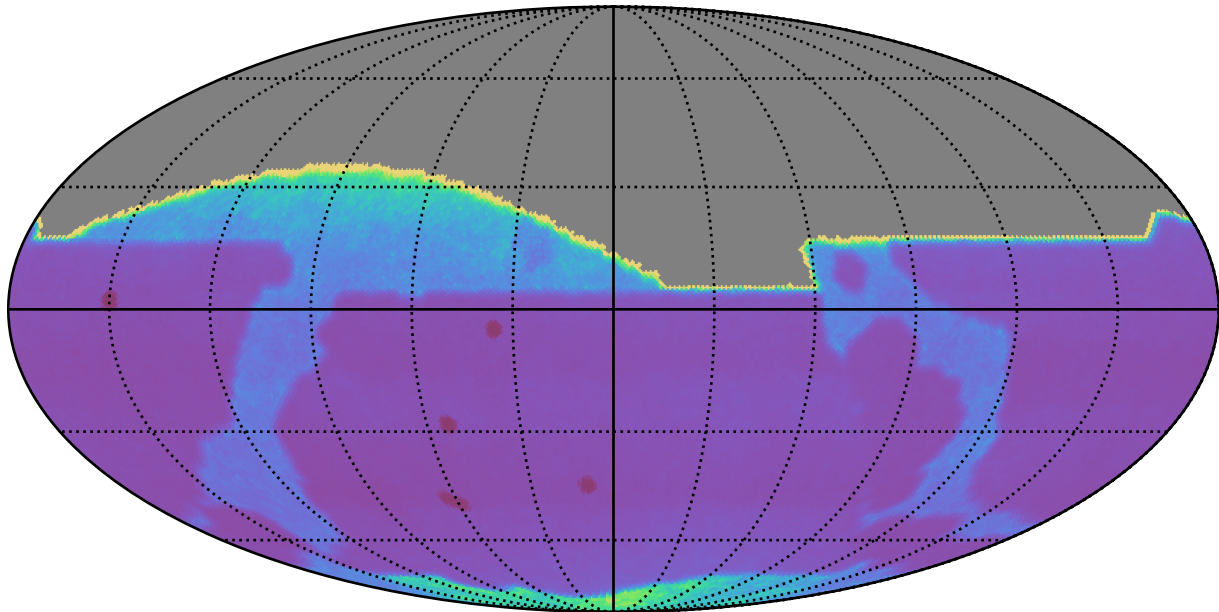
too_elab_r64_d3_gz_v3.4_10yrs : Proper Motion Uncert @ 20.5
