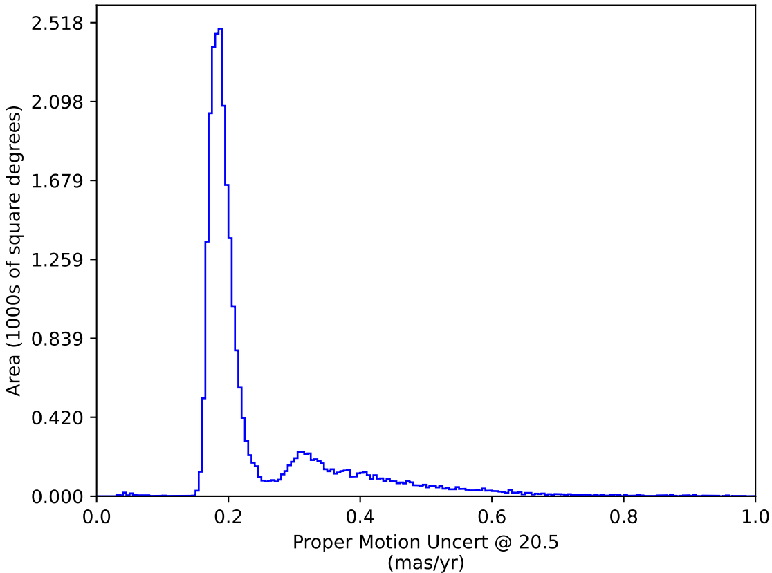
too_elab_r64_d3_gz_v3.4_10yrs : Proper Motion Uncert @ 20.5
