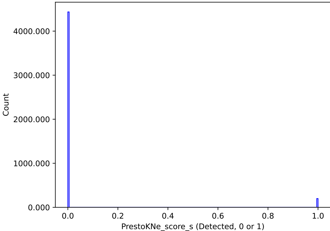
too_elab_r64_d3_gz_v3.4_10yrs : PrestoKNe_score_s
