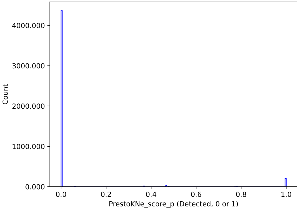
too_elab_r64_d3_gz_v3.4_10yrs : PrestoKNe_score_p
