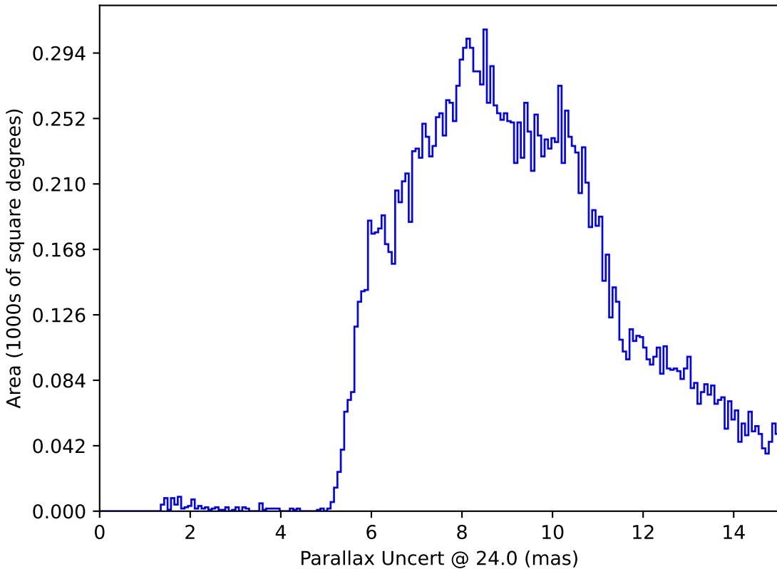
too_elab_r64_d3_gz_v3.4_10yrs : Parallax Uncert @ 24.0
