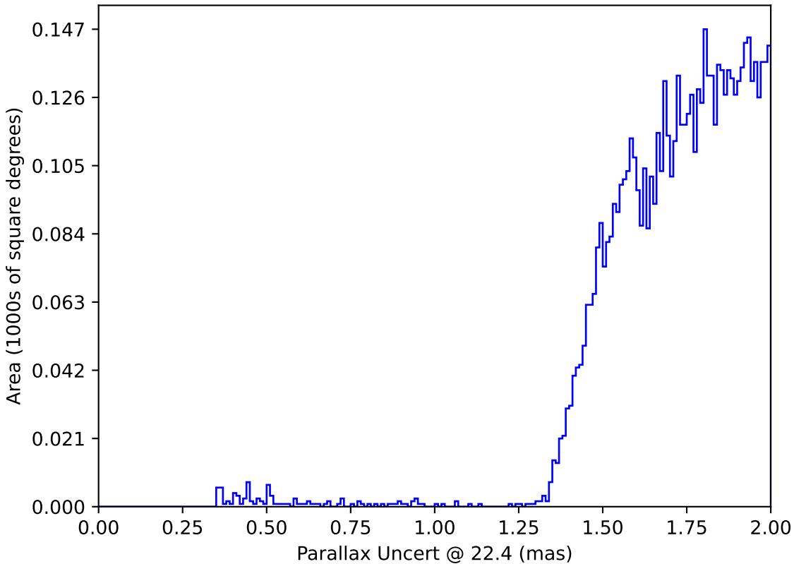
too_elab_r64_d3_gz_v3.4_10yrs : Parallax Uncert @ 22.4
