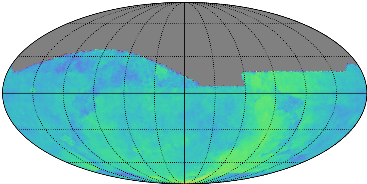
too_elab_r64_d3_gz_v3.4_10yrs : Parallax Coverage @ 24.0
